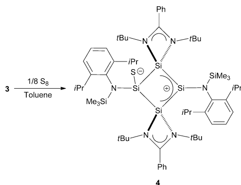
Scheme 3. Synthesis of 4 .
