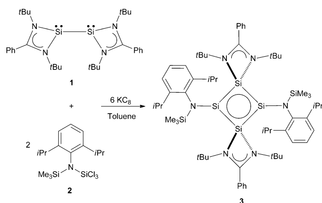
Scheme 1. Synthesis of 3 .
